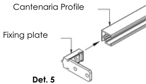
Cantenaria Profile
