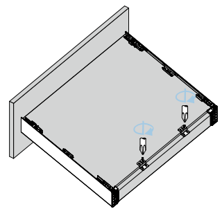
Fixing-brackets assembly
