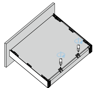
Fixing-brackets assembly
